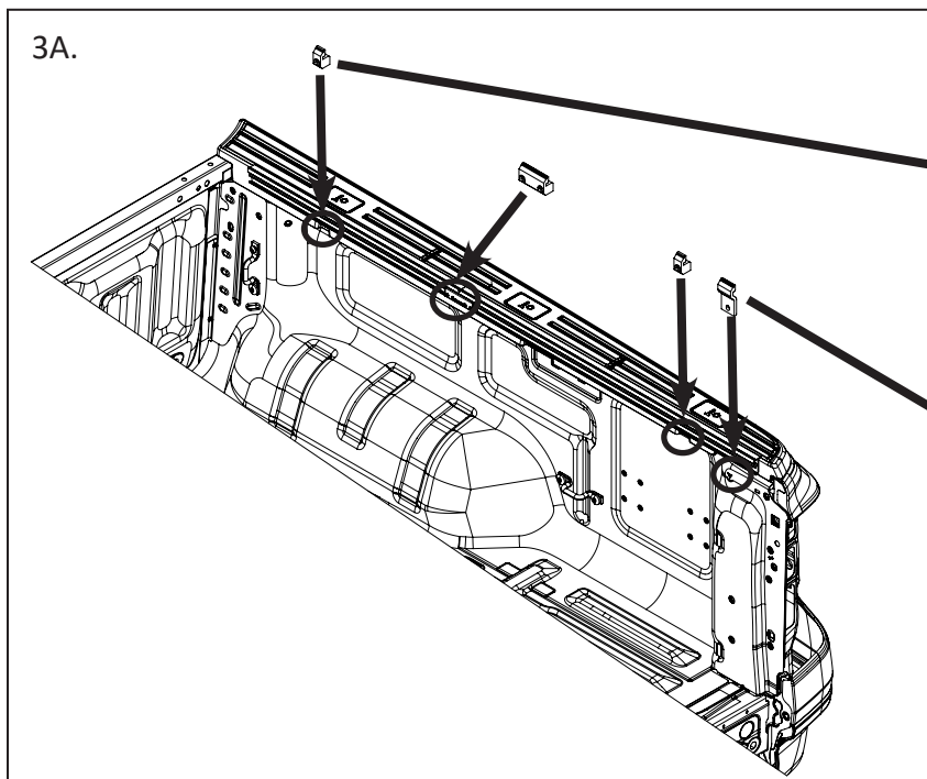
3A. 3B. 3C. Install clamps (CP) | Instalar abrazaderas | Installer les attaches
