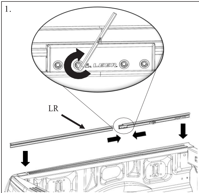
1. Connect split rail (LR, RR) | Conecte el riel dividid | Connecter le rail fendu
