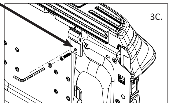
3A. 3B. 3C. Install clamps (CP) | Instalar abrazaderas | Installer les attaches
